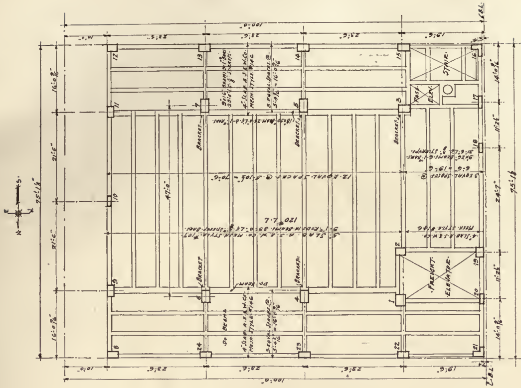
TYPICAL FRAMING PLAN. SCALE: 1/8" = 1'-0"
